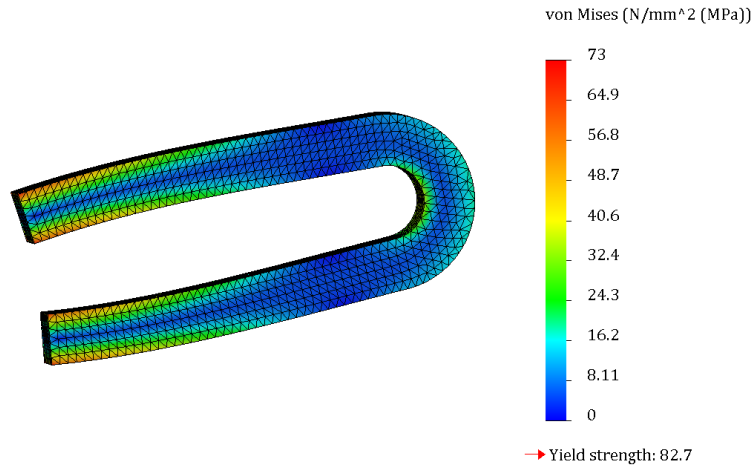
Figure 4-4: FEA analysis of the U shaped spring undergoing a moment of 52.5Nm .
