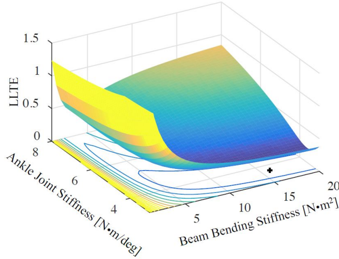
Figure 3-5: LLTE values calculated for each conceptual model foot over ranges of design variables. The optimal designs are those which produce the minimum LLTE, indicated here by the cross.
