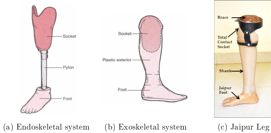
Figure 1-5: Drawing of typical trans-tibial prostheses [3] and photograph of a Jaipur Leg distributed in BMVSS
