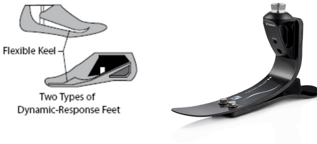
Figure 2-3: Two ESAR feet schematics examples along with Ossur's Flex-Foot sold at $1099 [6, 4].
