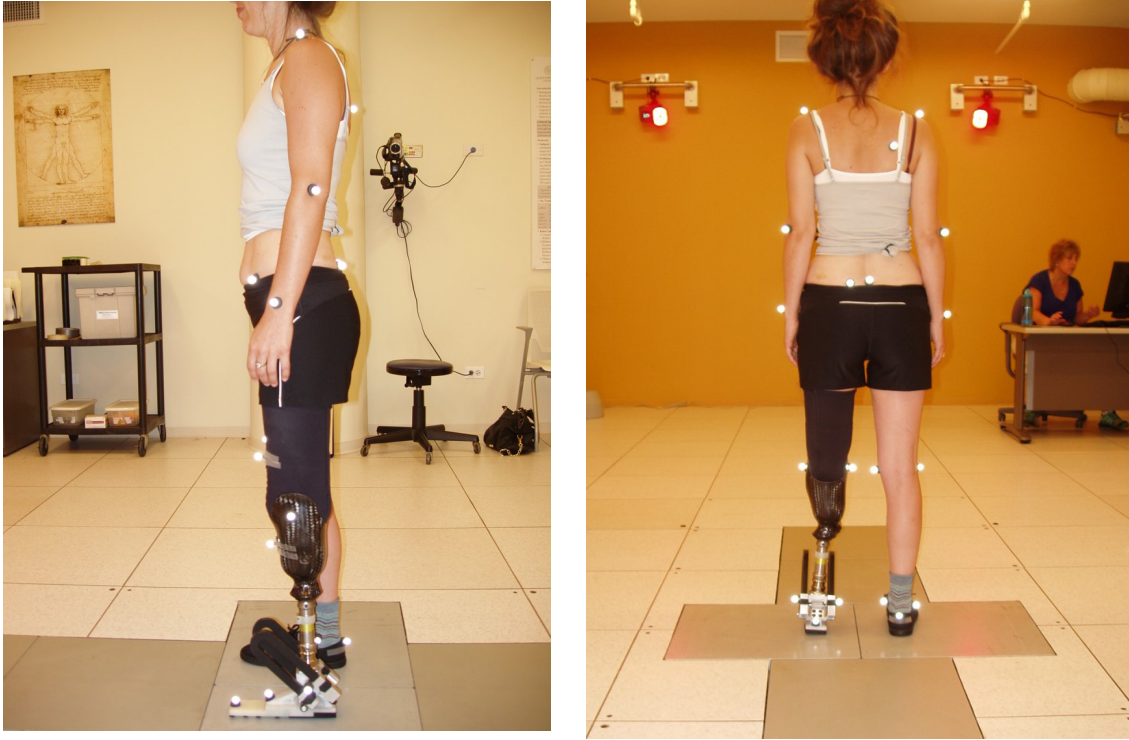
Figure 5-4: Gait lab setup and marker positions on the transtibial subject standing on the force plates and testing the prosthetic foot prototype with k_{ank} = 3.7 \text{ Nm/deg} .
