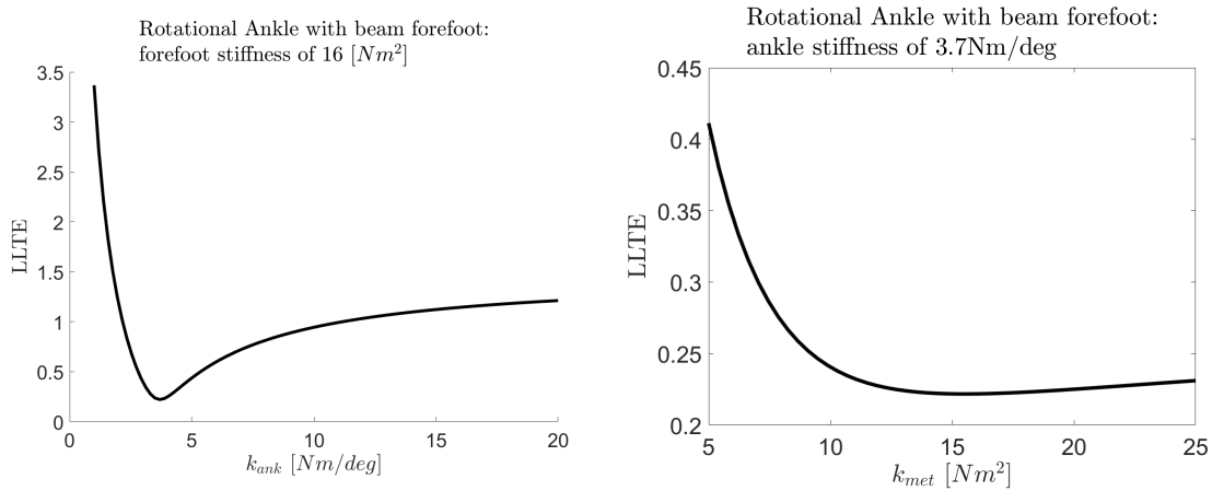
Figure 3-6: (a) Dependence of the LLTE value on the ankle rotational stiffness for k_{met} = 16.0 Nm 2 . (b) Dependence of the LLTE value on the forefoot beam stiffness for k_{ank} = 3.7 Nm/deg. The minimum LLTE value is achieved for k_{ank} = 3.7 Nm/deg and k_{met} = 16.0 Nm 2 .
